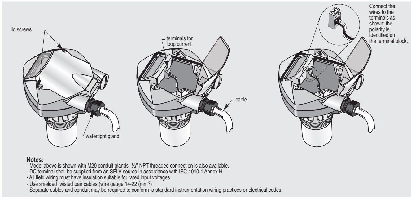
Fig. 4/3 SITRANS Probe LU connections
